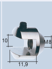
Halter, vertikal | 1 Vertical holder Support vertical
