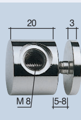
Glashalter | 1 Vertical panel holder Support de tablette en verre
