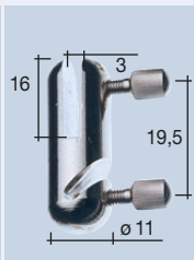
Stoffhalter | 1 Fabric holder Support tissu
