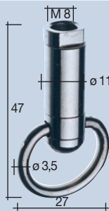
Ringhalter | 1 Ring holder Porte-anneau
