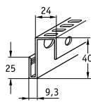
Connection profile
