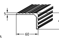
Cover angle
