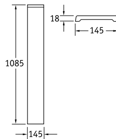
Neckar profile
