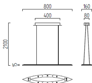
10 x 3W, LED warm weiß / warm white ca. 2900 K, 2700 Lumen 106/1400.17
