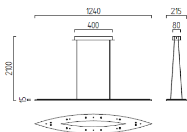
12 x 3W, LED warm weiß / warm white ca. 2900 K, 3240 Lumen 126/1400.17
