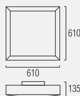
15-0591-S2-M1 4 x 2G11 36W ENERGY SAVING included
