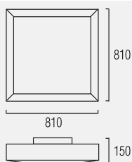
15-0592-S2-M1 4 x 2G11 55W ENERGY SAVING included
