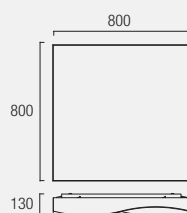
15-2781-S2-M1 2G11 4x55W ENERGY SAVING included
