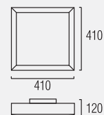
15-0590-S2-M1 4 x 2G11 18W ENERGY SAVING included
